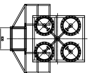
FRONT VIEW OF BURNER
